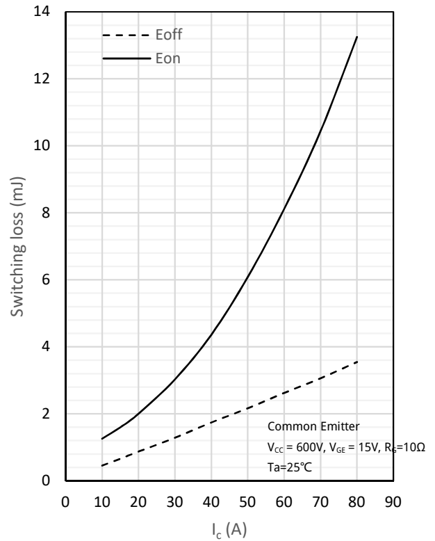
Fig. 6 Switching loss vs. collector current
