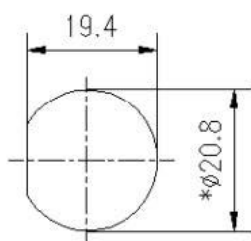
Panel Cut-Out
