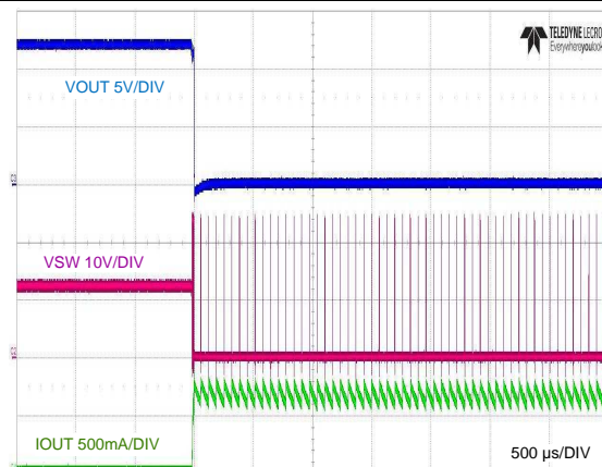
Figure 20. Full-Load Start-up and Shutdown with EN/UVLO
